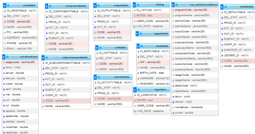
Gambar 6. Class Diagram
