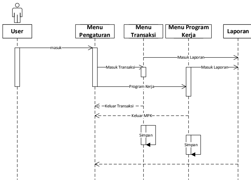
Gambar 5. Sequences Diagram
