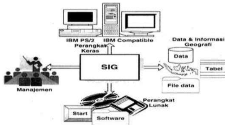
Gambar 2. Conceptual Framework
